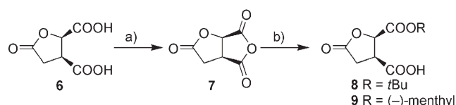
Scheme 3. Formation of 7 and its regioselective opening: a) Ac 2 O, 160 °C, 15 min, 85%; b) for 8 : anhydrous t BuOH, reflux, 15 h, quant.; for 9 : (1 R ,2 S ,5 R )-(-)-menthol, 100 °C, 36 h, 27%.
