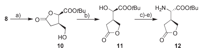
Scheme 4. Transformation and rearrangement of 8 : a) BH 3 /THF, THF, 0 °C → RT, 5 h, 88%; b) H + , 78%; c) methanesulfonyl chloride, pyridine, CH 2 Cl 2 , 24 h; d) NaN 3 , DMF, 47% over two steps; e) Pd/C, H 2 , EtOAc, 8 h, 90%.
