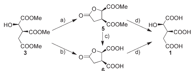
Scheme 2. Conversion of 3 : a) 10 mol % para -toluenesulfonic acid, toluene, reflux, 80%; b) 4.0 M HCl, reflux, 8 h, quant.; c) 1.0 M HCl, reflux, 4 h, quant.; d) 3 equiv NaOH, amberlite IR-120, quant.
