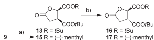
Scheme 6. a) 2-Methylpropene, cat. H 2 SO 4 , CH 2 Cl 2 , 48 h, quant.; b) inversion of the conformation at C3 for 16 : DBU, CH 2 Cl 2 , 50 °C, 30 min, 80% (based on recovered starting material); for 17 : DBU, CH 2 Cl 2 , 50 °C, 1 h, 89% (based on recovered starting material). DBU = 1,8-diazabicyclo[5.4.0]undec-7-ene.
