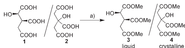
Scheme 1. Esterification of the concentrated fermentation broth: a) MeOH, 2,2-dimethoxypropane, 10 mol% trimethylsilyl chloride, 3 days, RT, 80–88%.
