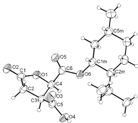
Figure 1. Crystal structure of 9 . [6]
